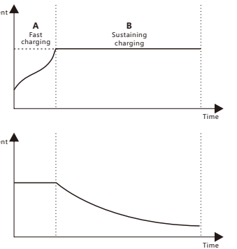
Fig. 1-6 LI Battery charging stages diagram
